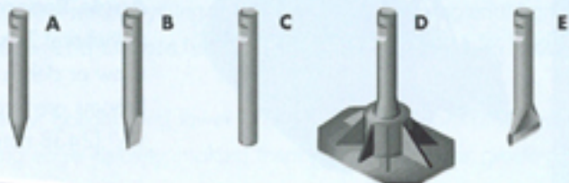
A. Moil (Conical) Point B. Cross-Cut Chisel C. Blunt Tool D. Tamping Pad E. Asphalt Cutter
